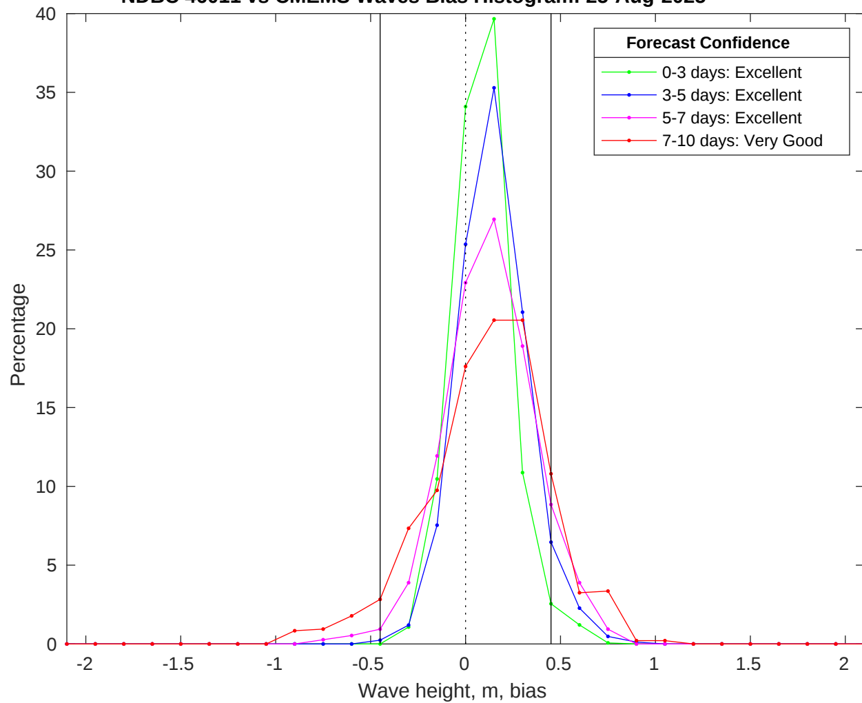
NDBC 46011 vs CMEMS Waves Bias Histogram: 25-Aug-2025
