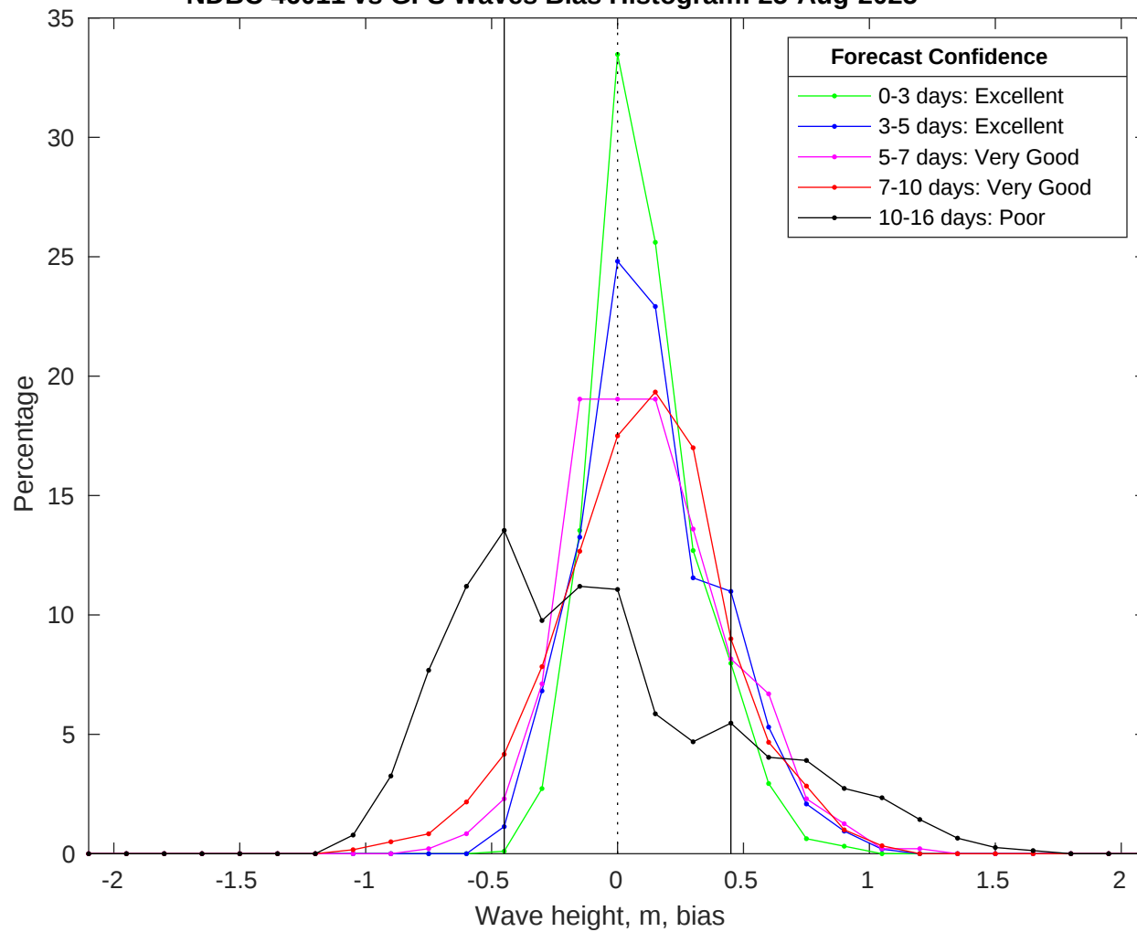
NDBC 46011 vs GFS Waves Bias Histogram: 25-Aug-2025
