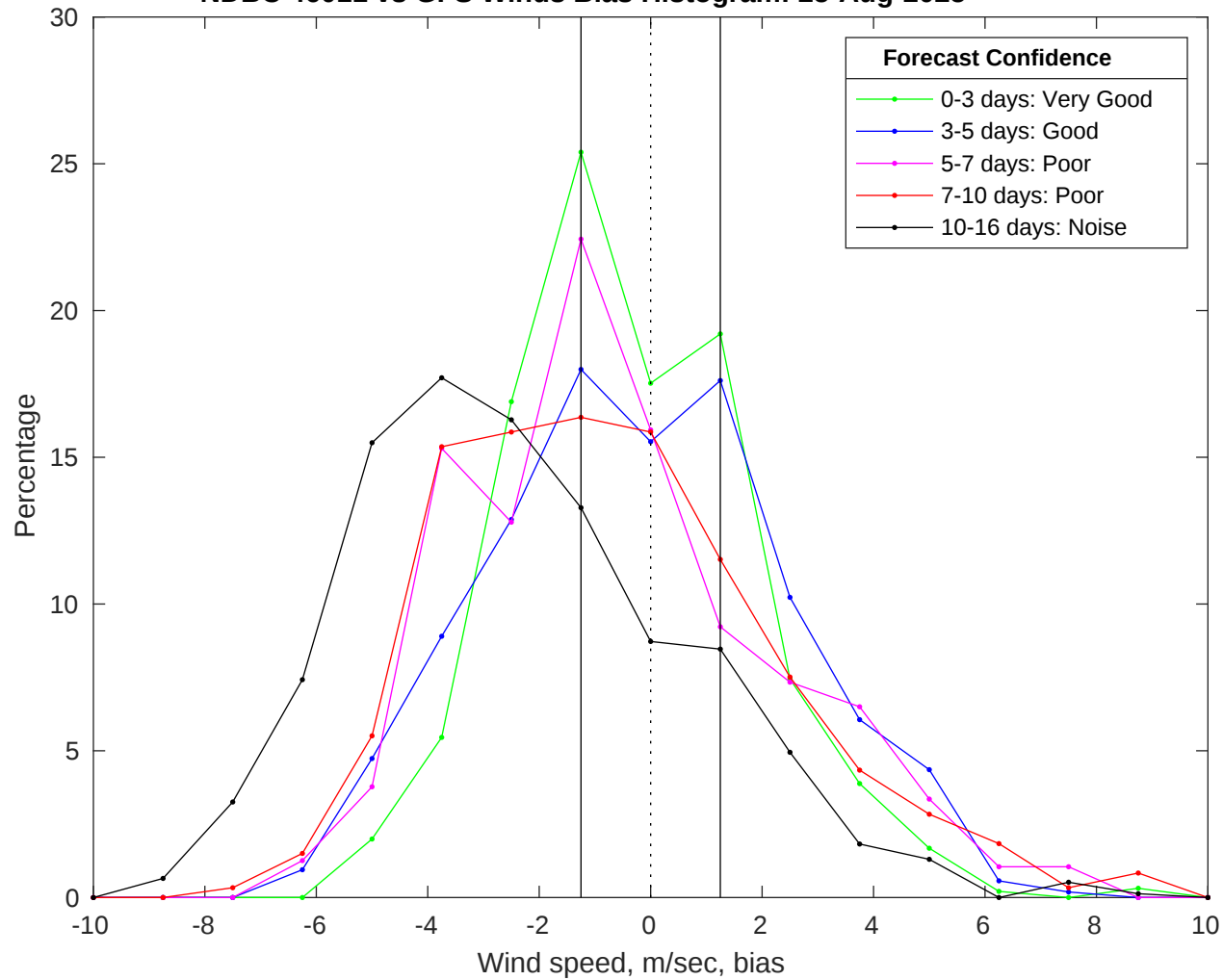
NDBC 46011 vs GFS Winds Bias Histogram: 25-Aug-2025
