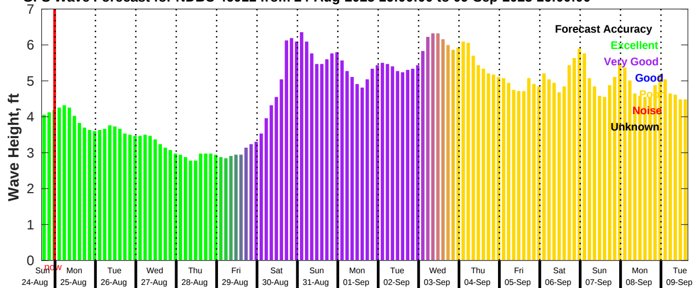
GFS Wave Forecast for NDBC 46011 from 24-Aug-2025 16:00:00 to 09-Sep-2025 16:00:00
