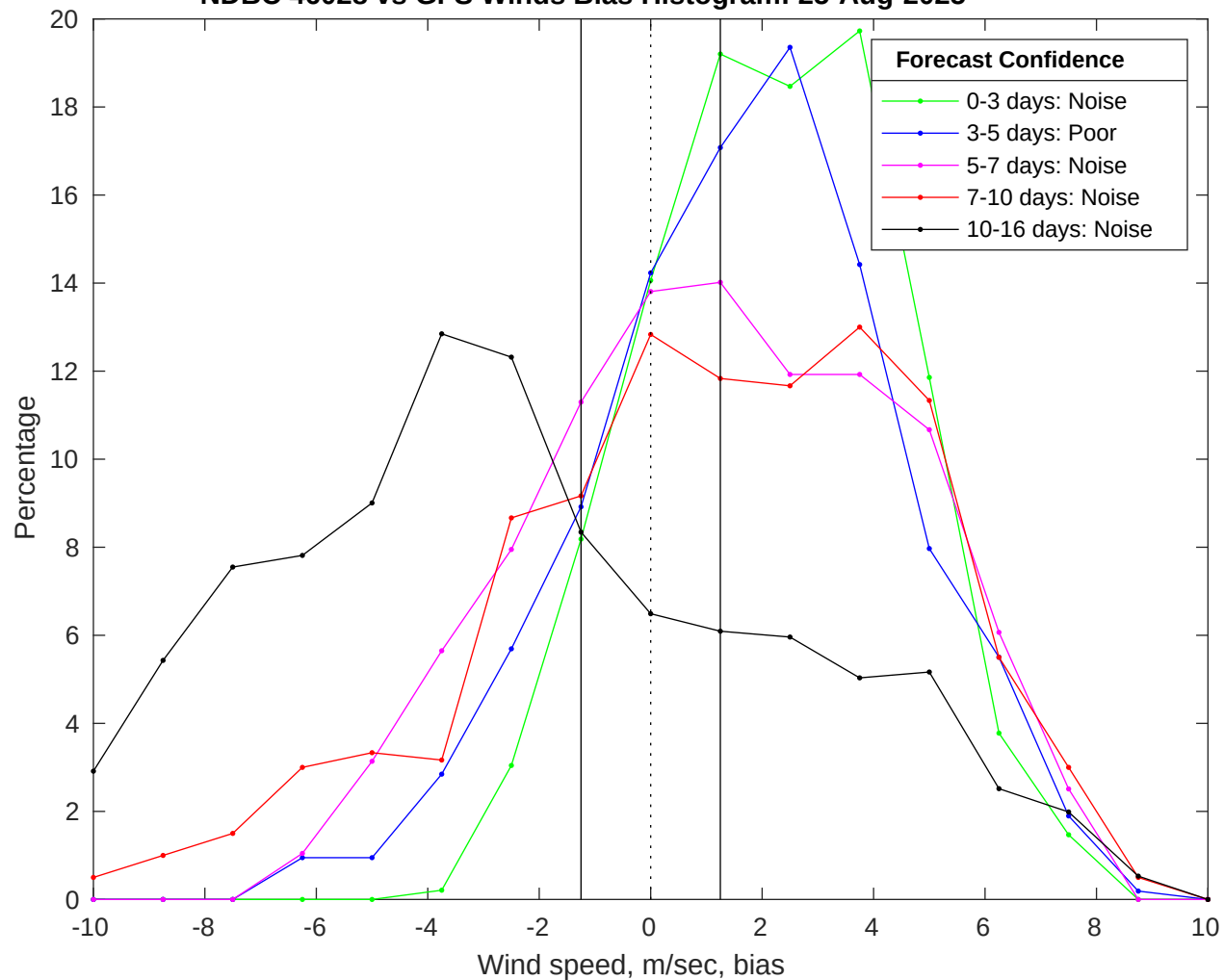
NDBC 46028 vs GFS Winds Bias Histogram: 25-Aug-2025
