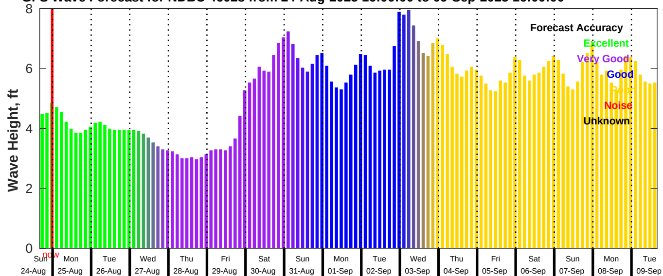
GFS Wave Forecast for NDBC 46028 from 24-Aug-2025 16:00:00 to 09-Sep-2025 16:00:00
