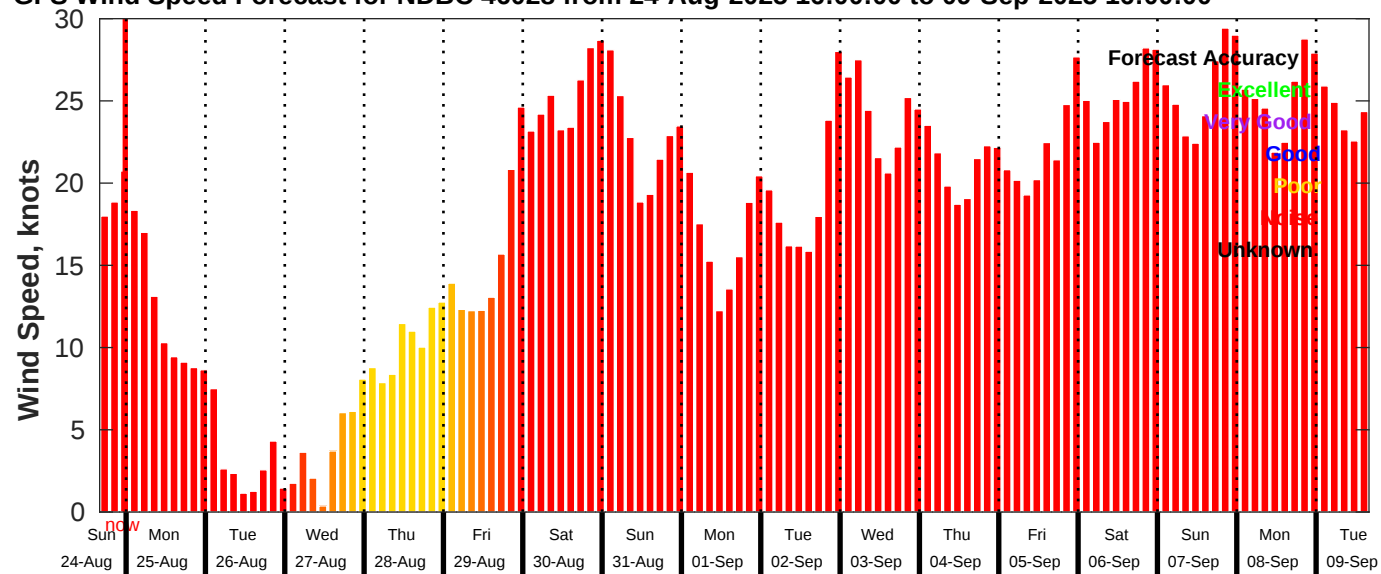
GFS Wind Speed Forecast for NDBC 46028 from 24-Aug-2025 16:00:00 to 09-Sep-2025 16:00:00
