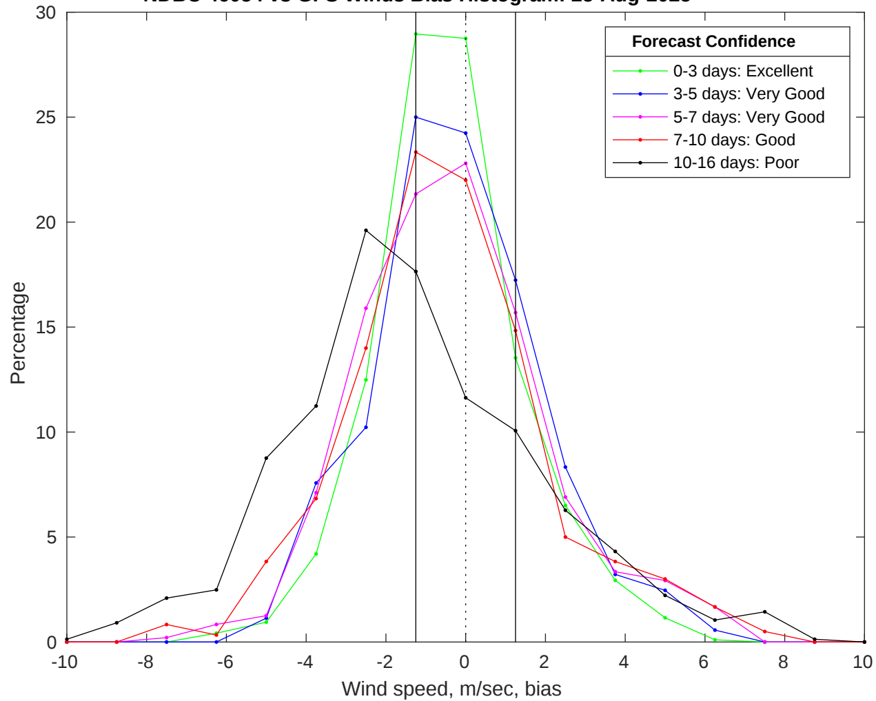
NDBC 46054 vs GFS Winds Bias Histogram: 25-Aug-2025
