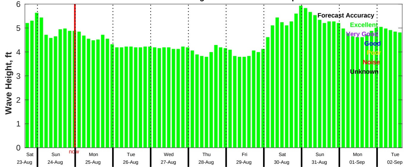
CMEMS Wave Forecast for NDBC 46054 from 23-Aug-2025 16:00:00 to 02-Sep-2025 16:00:00
