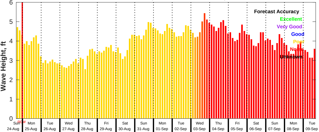
GFS Wave Forecast for NDBC 46054 from 24-Aug-2025 16:00:00 to 09-Sep-2025 16:00:00
