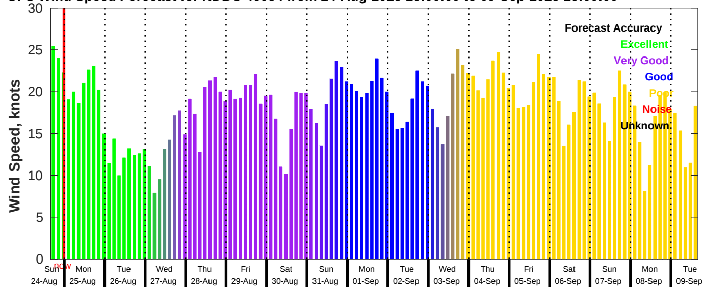
GFS Wind Speed Forecast for NDBC 46054 from 24-Aug-2025 16:00:00 to 09-Sep-2025 16:00:00
