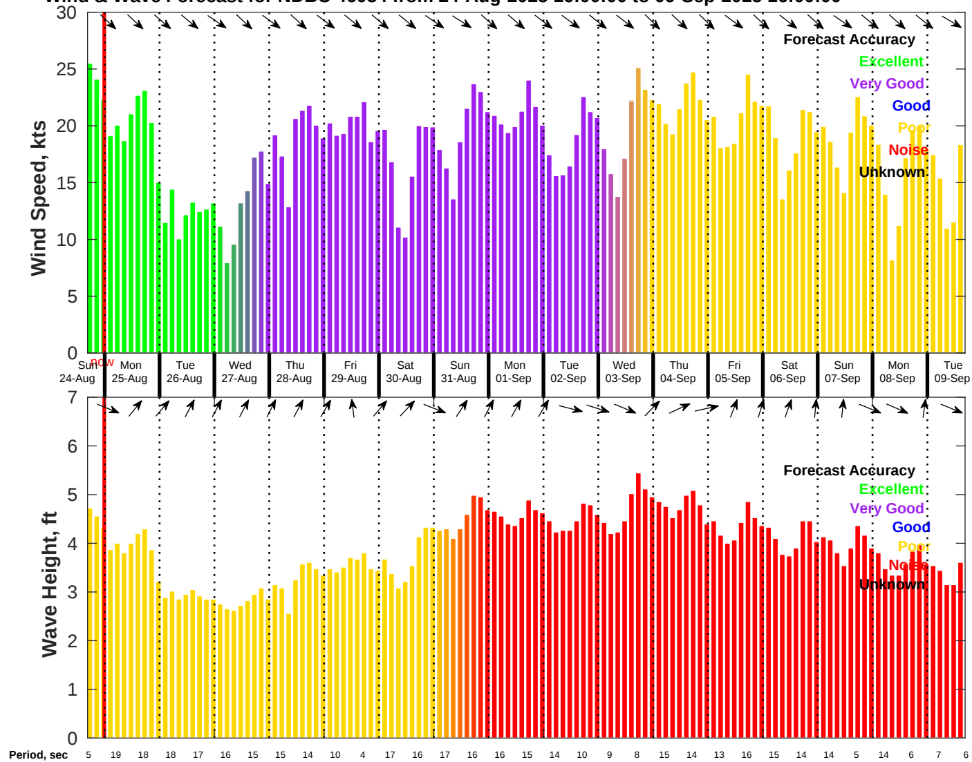
Wind & Wave Forecast for NDBC 46054 from 24-Aug-2025 16:00:00 to 09-Sep-2025 16:00:00
