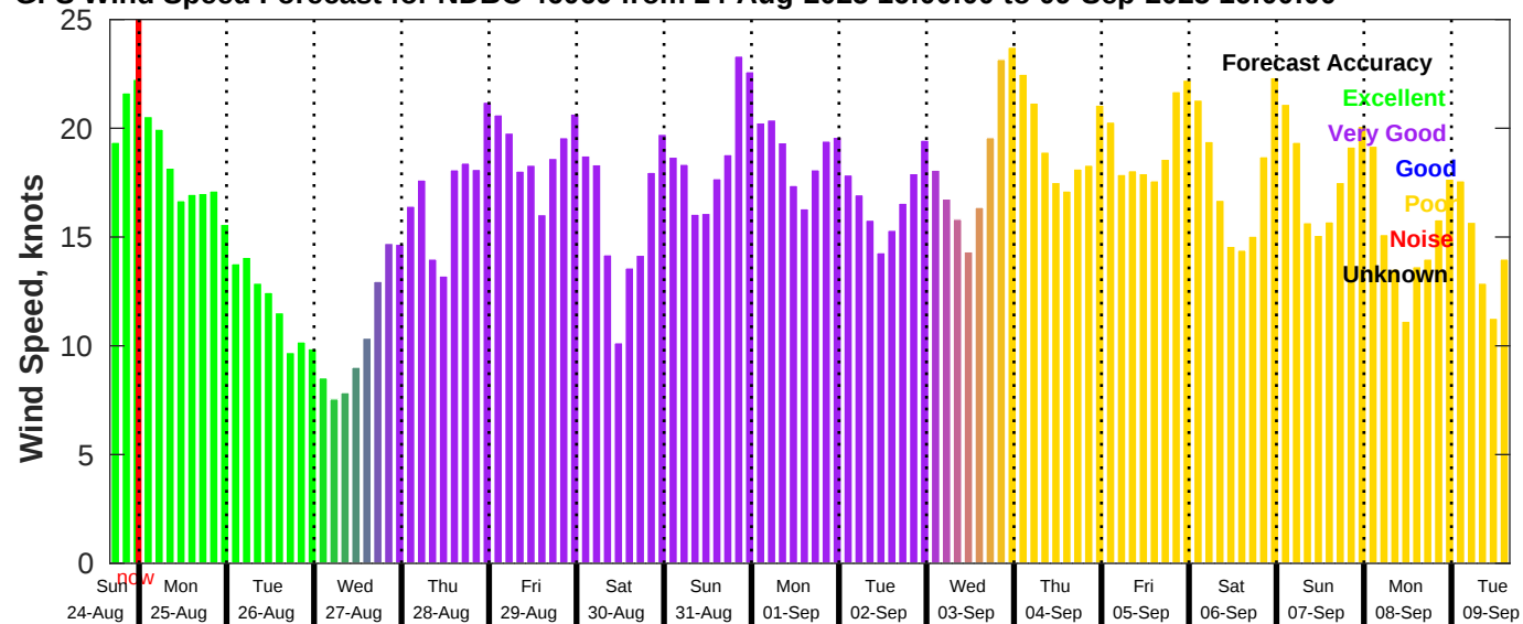
GFS Wind Speed Forecast for NDBC 46069 from 24-Aug-2025 16:00:00 to 09-Sep-2025 16:00:00
