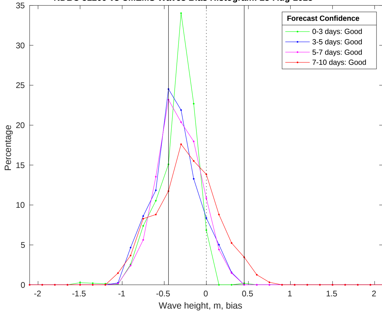
NDBC 51209 vs CMEMS Waves Bias Histogram: 25-Aug-2025
