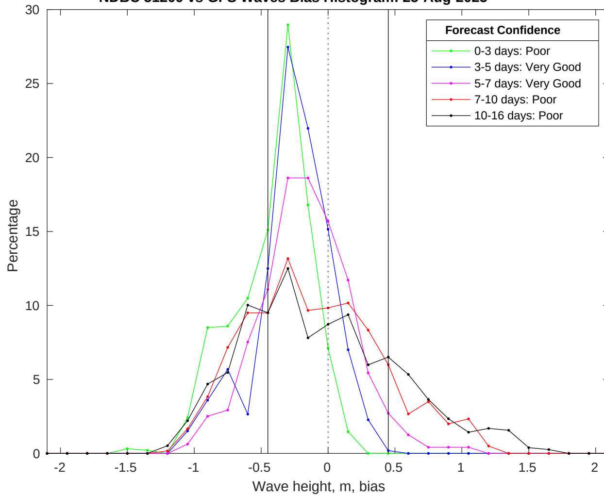
NDBC 51209 vs GFS Waves Bias Histogram: 25-Aug-2025
