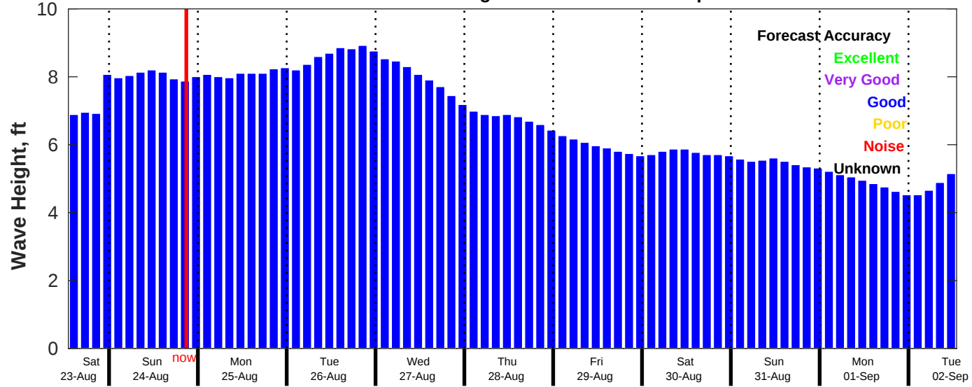
CMEMS Wave Forecast for NDBC 51209 from 23-Aug-2025 13:00:00 to 02-Sep-2025 13:00:00
