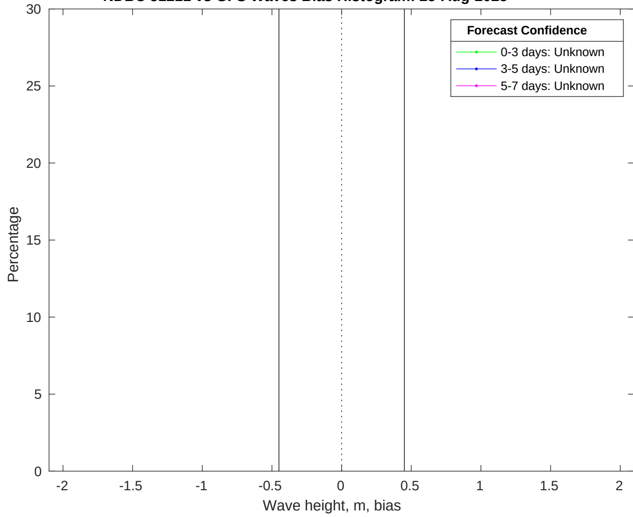
NDBC 51211 vs GFS Waves Bias Histogram: 25-Aug-2025
