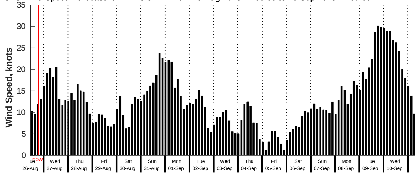
GFS Wind Speed Forecast for NDBC 52211 from 25-Aug-2025 11:00:00 to 10-Sep-2025 11:00:00
