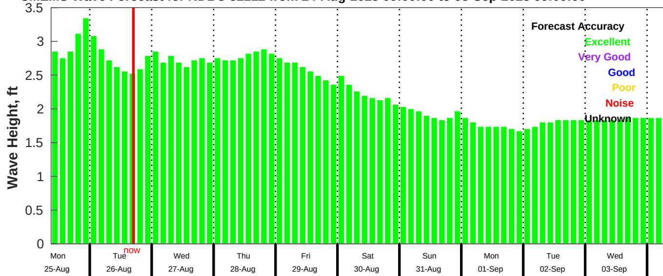
CMEMS Wave Forecast for NDBC 52212 from 24-Aug-2025 09:00:00 to 03-Sep-2025 09:00:00
