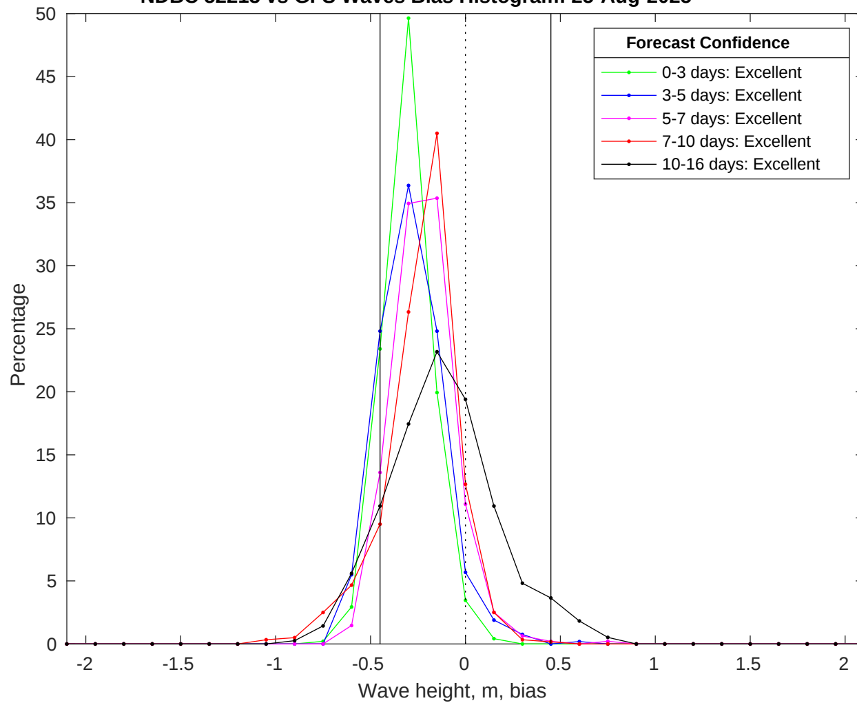
NDBC 52213 vs GFS Waves Bias Histogram: 25-Aug-2025
