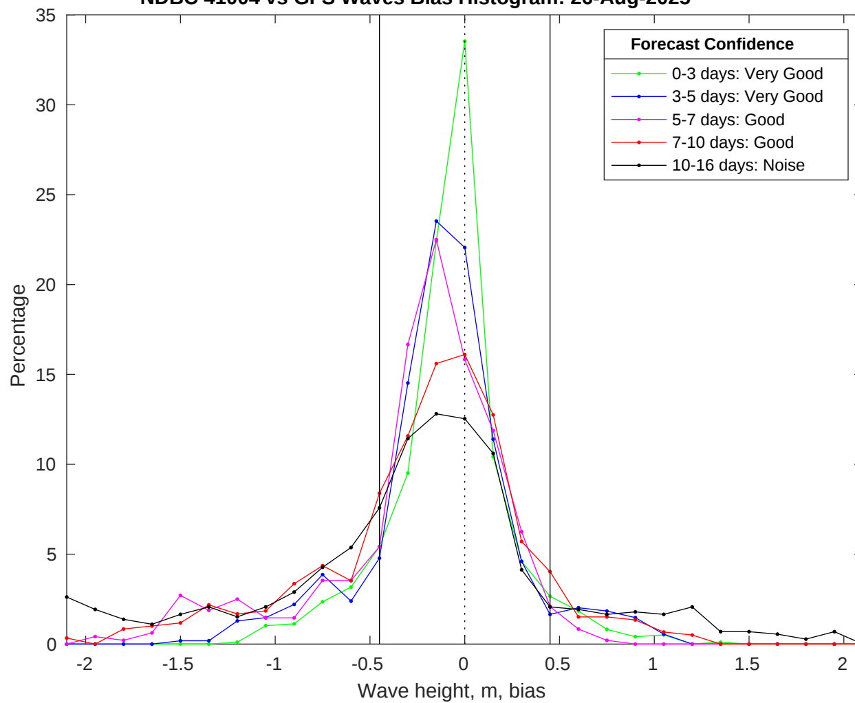
NDBC 41004 vs GFS Waves Bias Histogram: 26-Aug-2025
