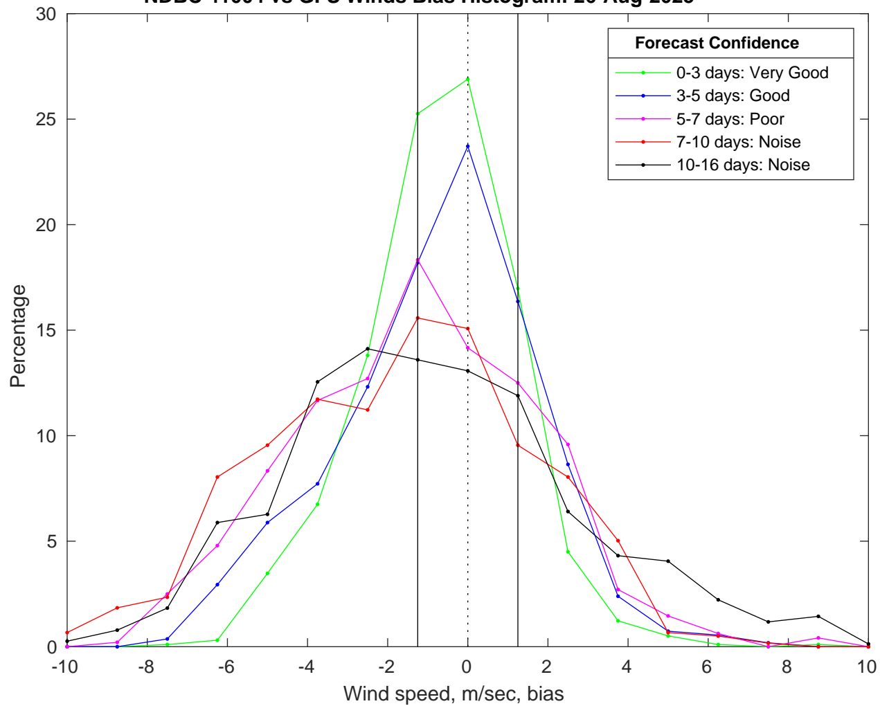
NDBC 41004 vs GFS Winds Bias Histogram: 26-Aug-2025
