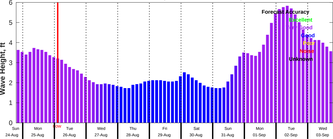
CMEMS Wave Forecast for NDBC 41004 from 24-Aug-2025 19:00:00 to 03-Sep-2025 19:00:00
