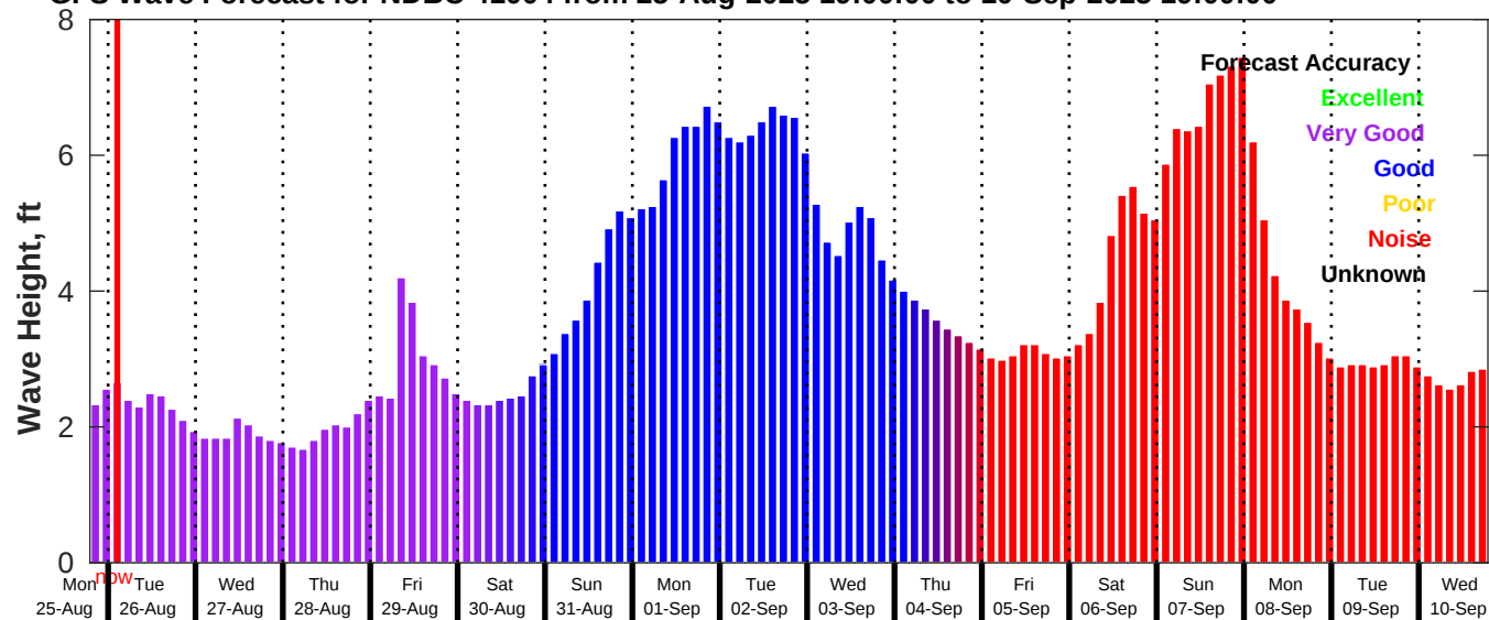
GFS Wave Forecast for NDBC 41004 from 25-Aug-2025 19:00:00 to 10-Sep-2025 19:00:00
