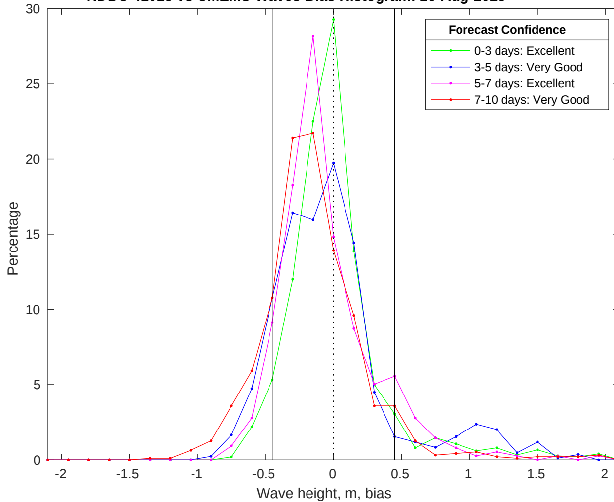
NDBC 41013 vs CMEMS Waves Bias Histogram: 26-Aug-2025
