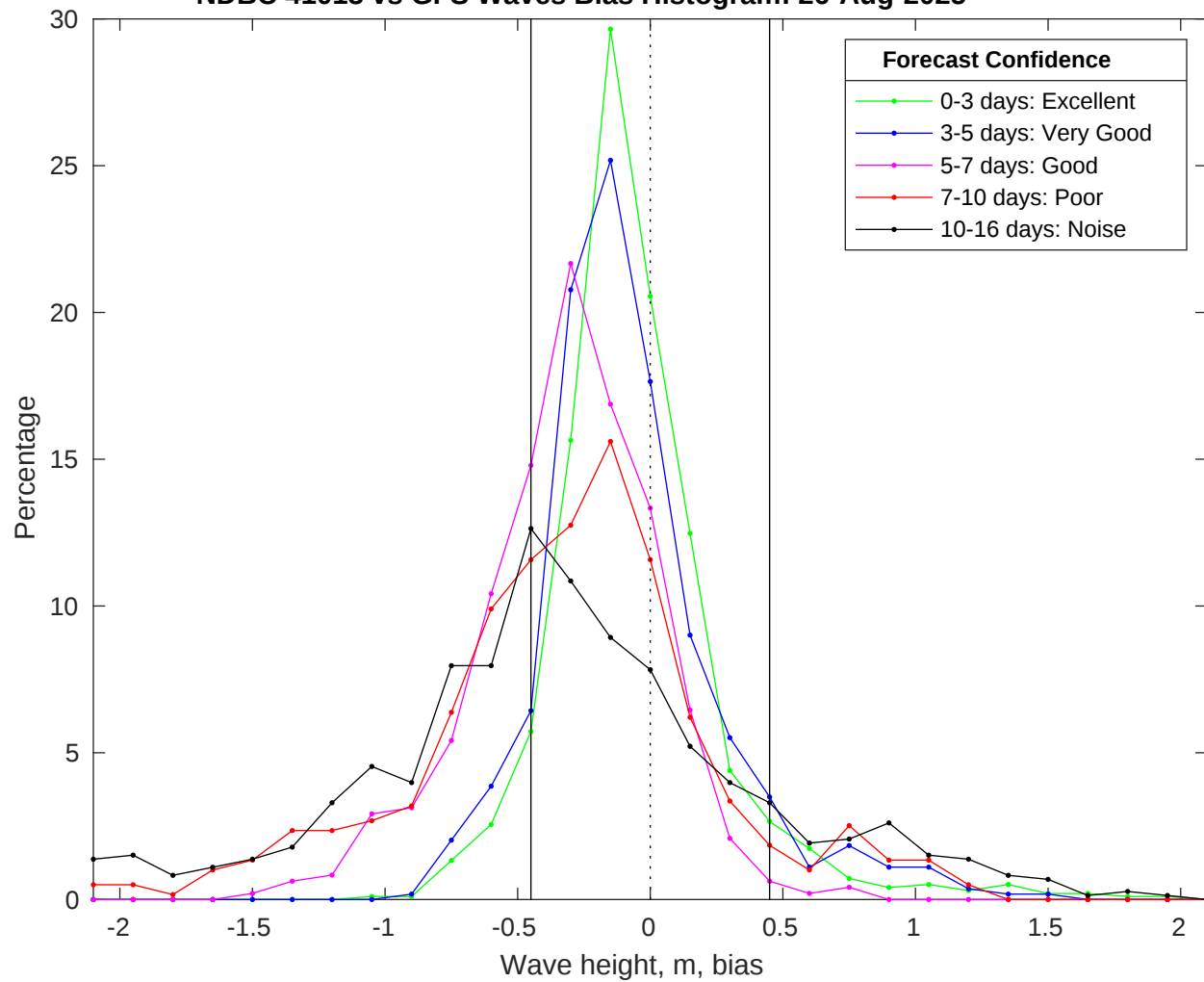
NDBC 41013 vs GFS Waves Bias Histogram: 26-Aug-2025
