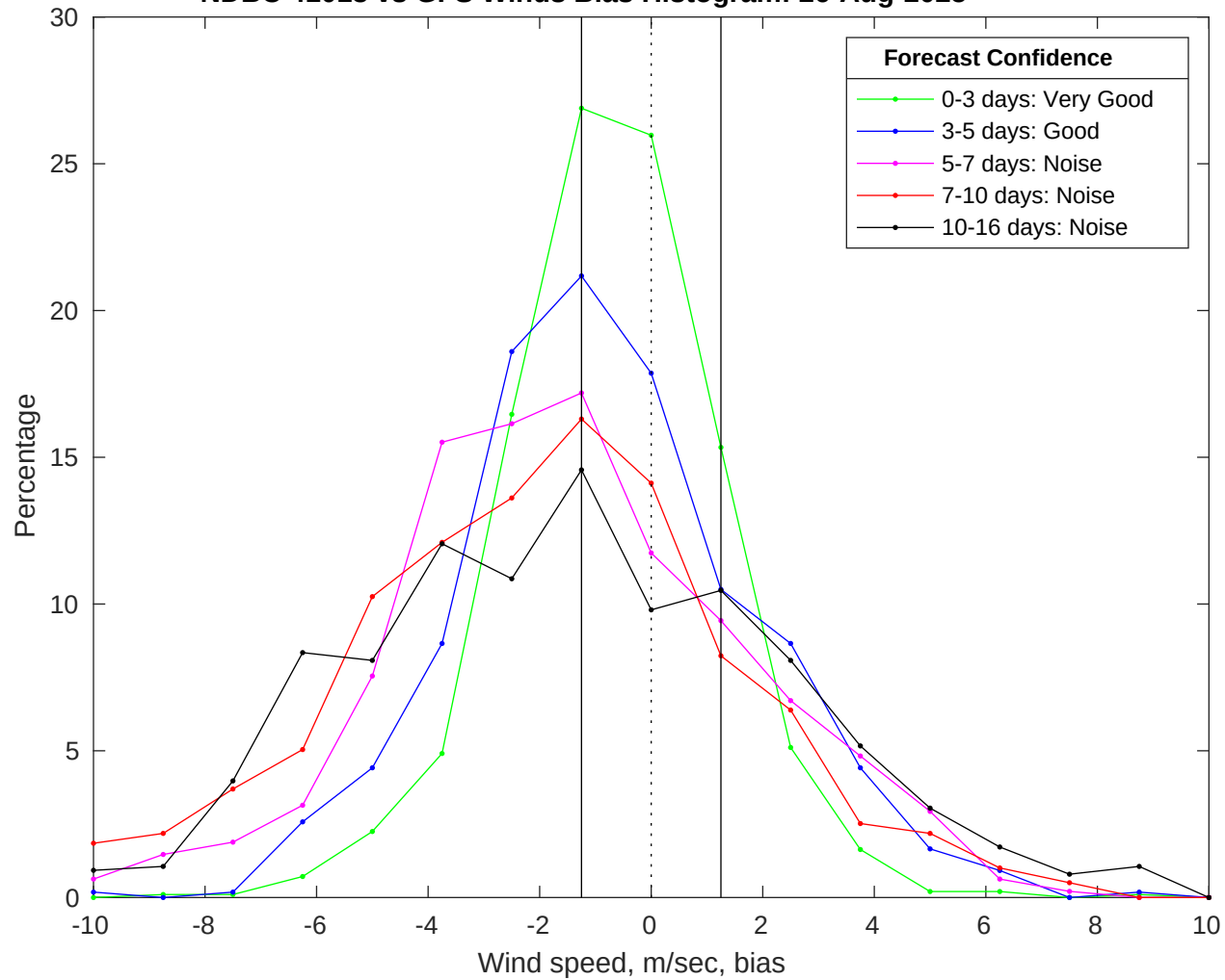
NDBC 41013 vs GFS Winds Bias Histogram: 26-Aug-2025
