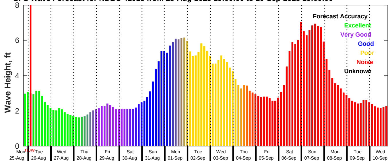
GFS Wave Forecast for NDBC 41013 from 25-Aug-2025 19:00:00 to 10-Sep-2025 19:00:00
