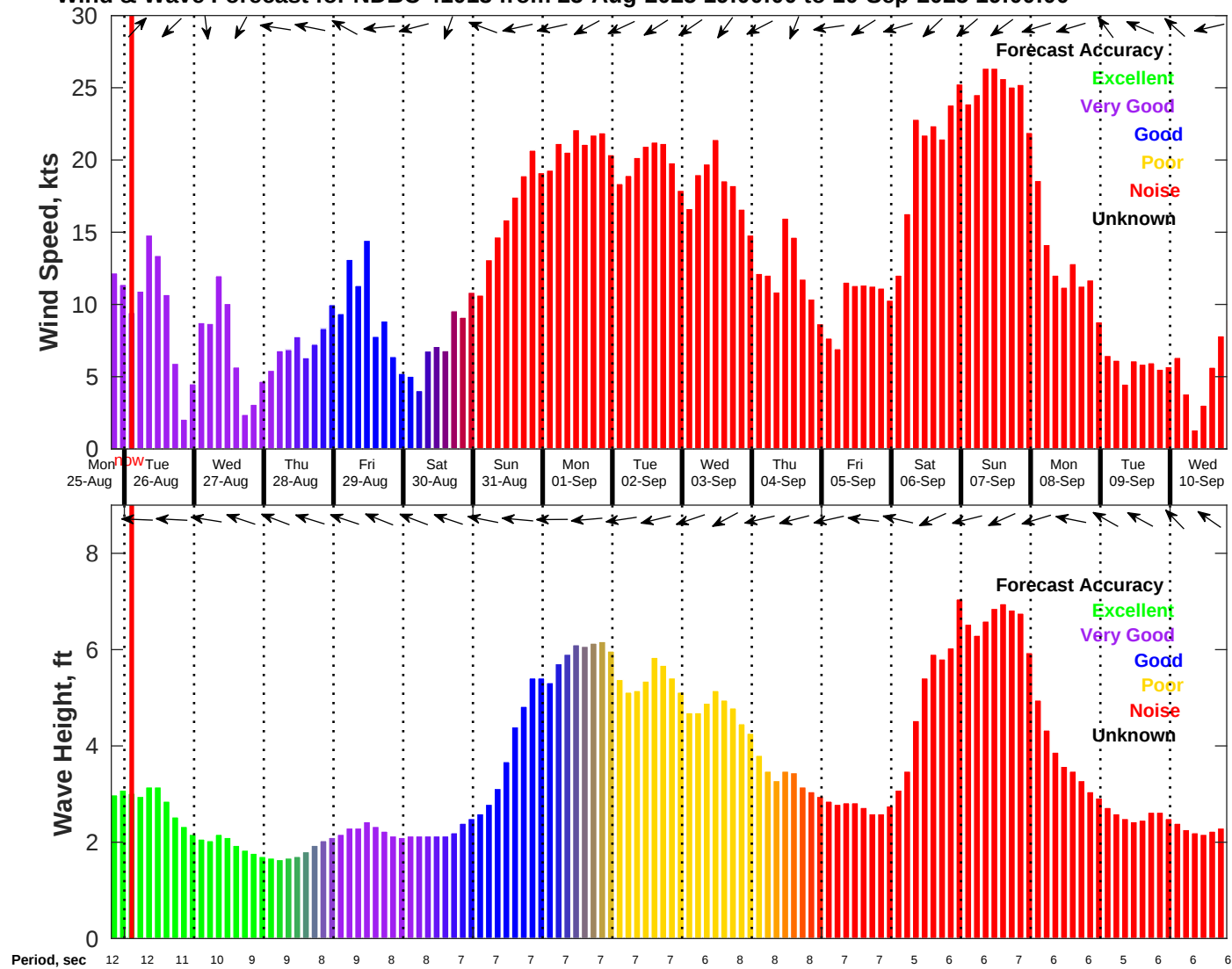
Wind & Wave Forecast for NDBC 41013 from 25-Aug-2025 19:00:00 to 10-Sep-2025 19:00:00
