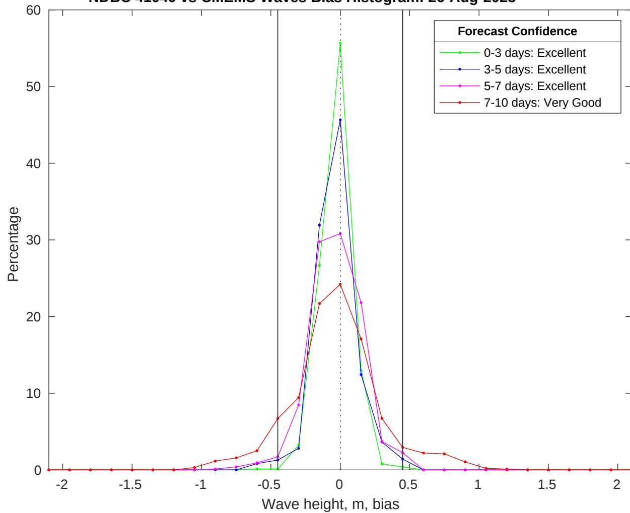
NDBC 41040 vs CMEMS Waves Bias Histogram: 26-Aug-2025
