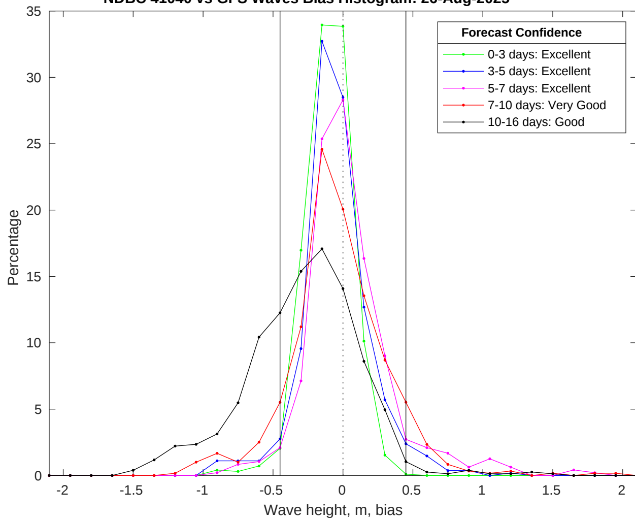
NDBC 41040 vs GFS Waves Bias Histogram: 26-Aug-2025
