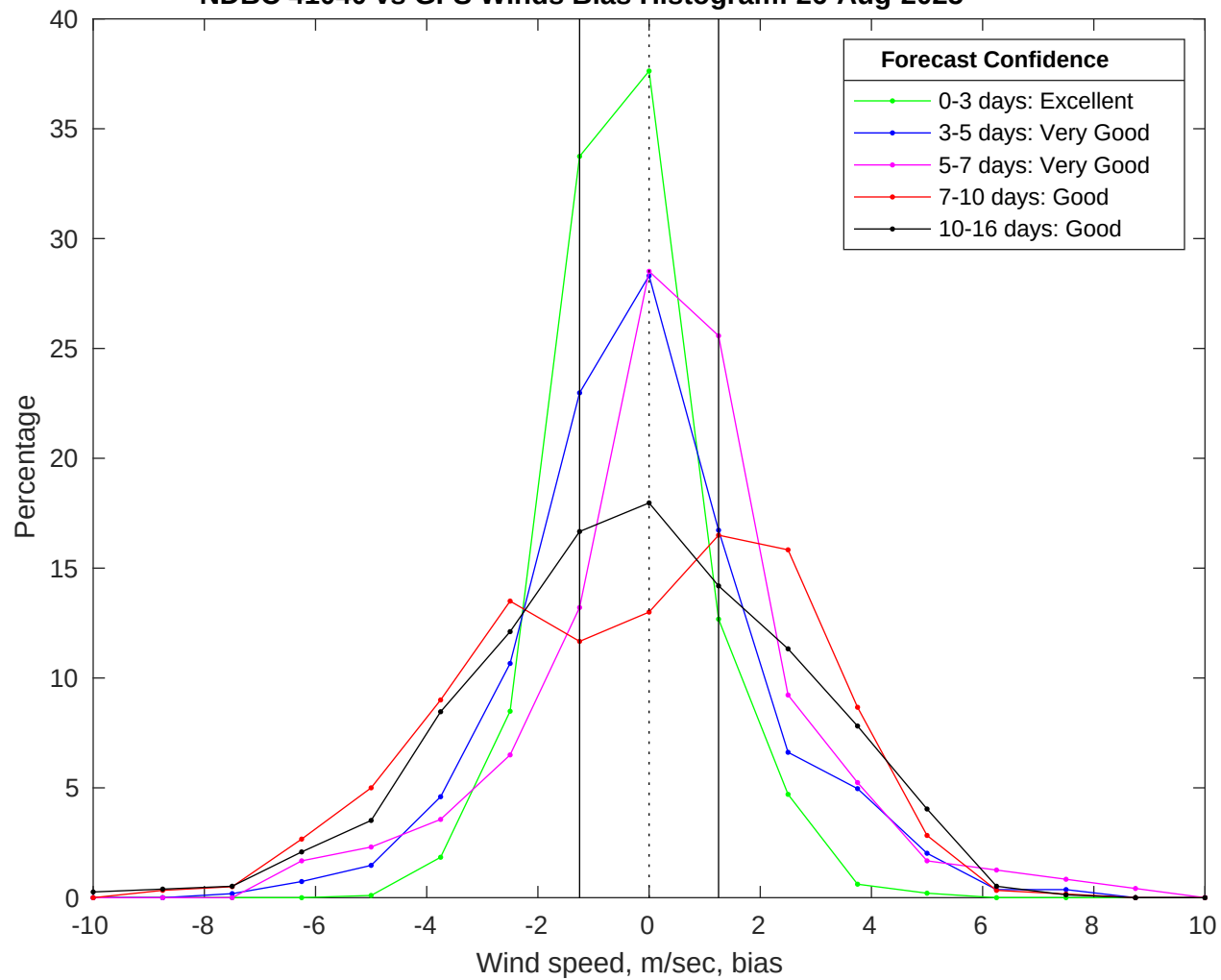
NDBC 41040 vs GFS Winds Bias Histogram: 26-Aug-2025
