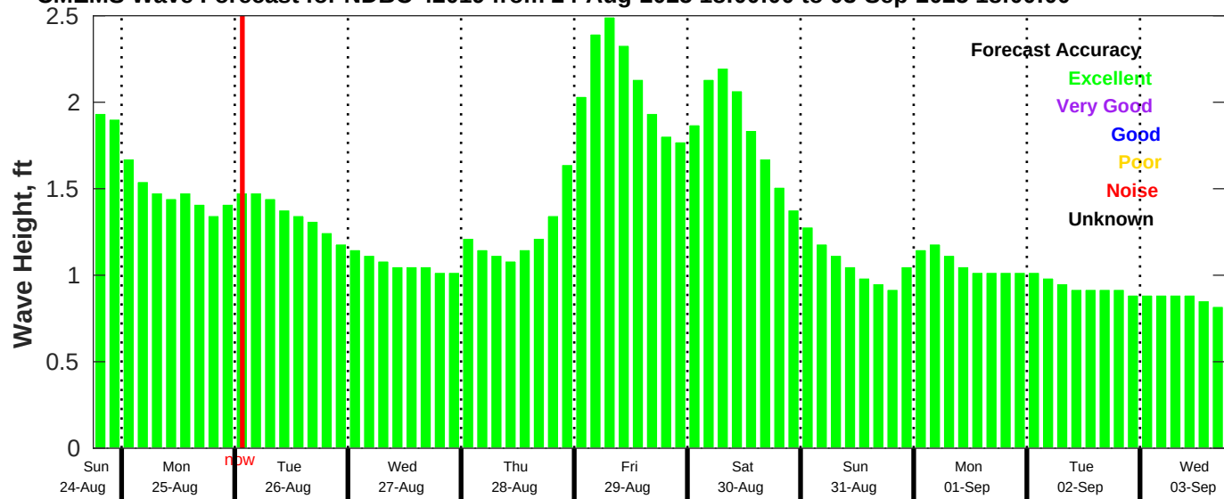
CMEMS Wave Forecast for NDBC 42019 from 24-Aug-2025 18:00:00 to 03-Sep-2025 18:00:00
