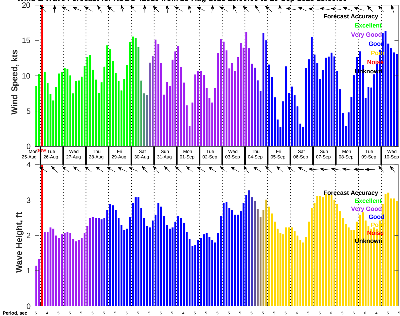
Wind & Wave Forecast for NDBC 42020 from 25-Aug-2025 18:00:00 to 10-Sep-2025 18:00:00
