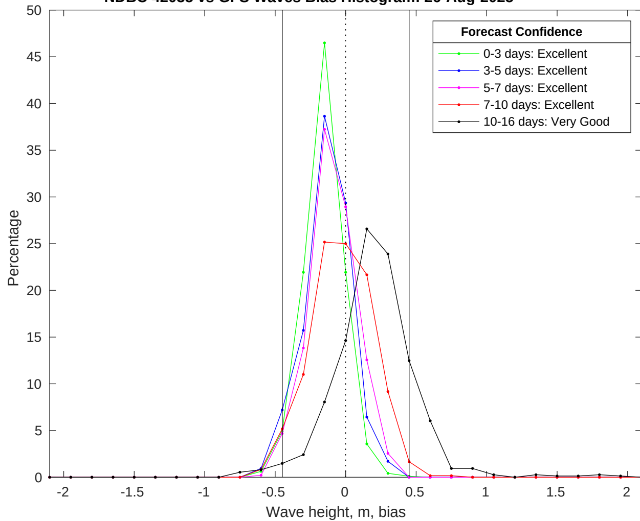
NDBC 42035 vs GFS Waves Bias Histogram: 26-Aug-2025
