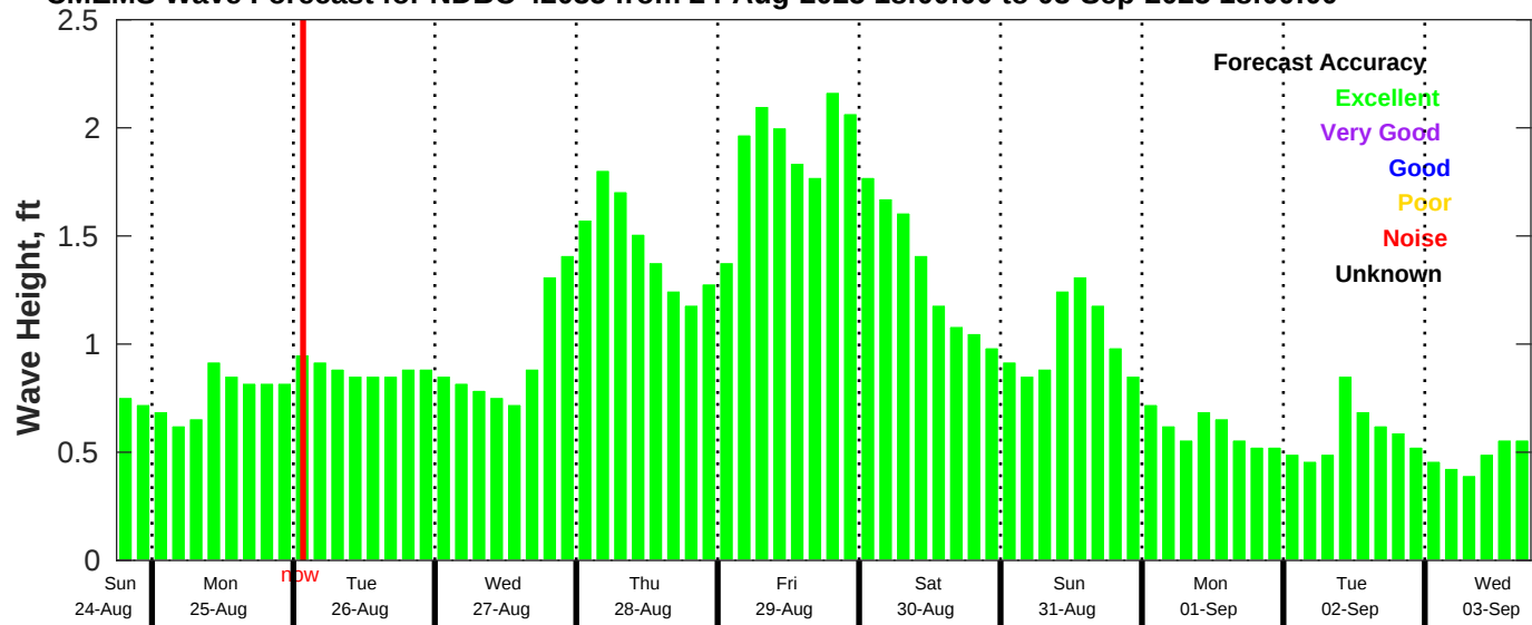
CMEMS Wave Forecast for NDBC 42035 from 24-Aug-2025 18:00:00 to 03-Sep-2025 18:00:00
