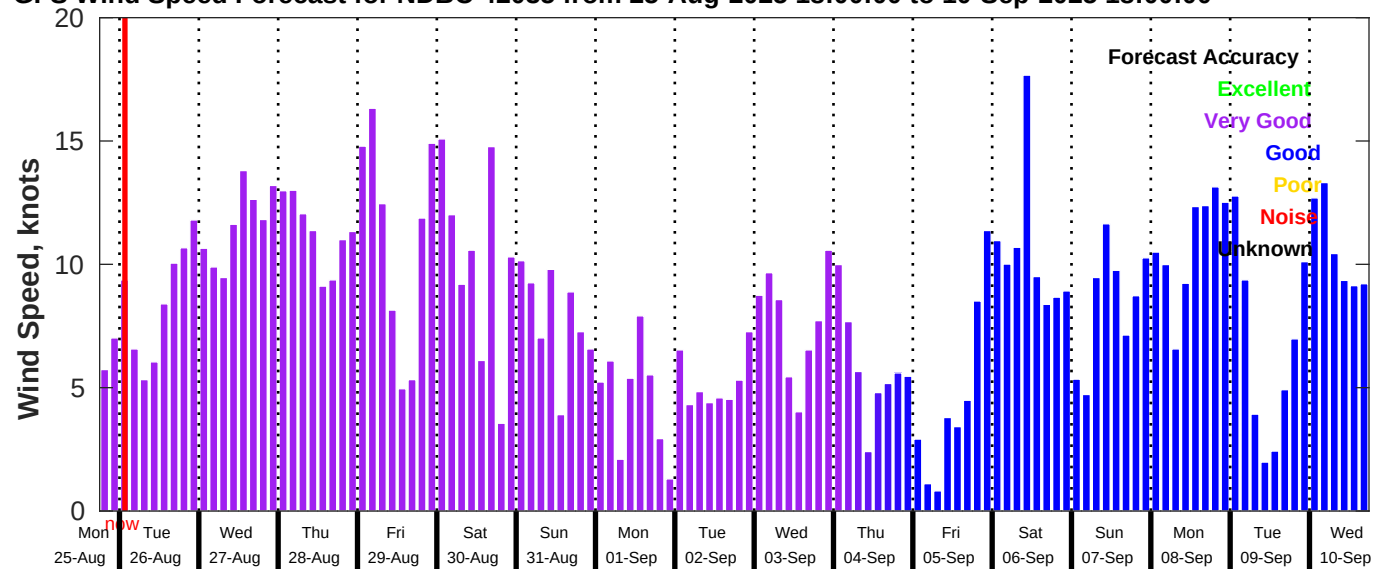
GFS Wind Speed Forecast for NDBC 42035 from 25-Aug-2025 18:00:00 to 10-Sep-2025 18:00:00
