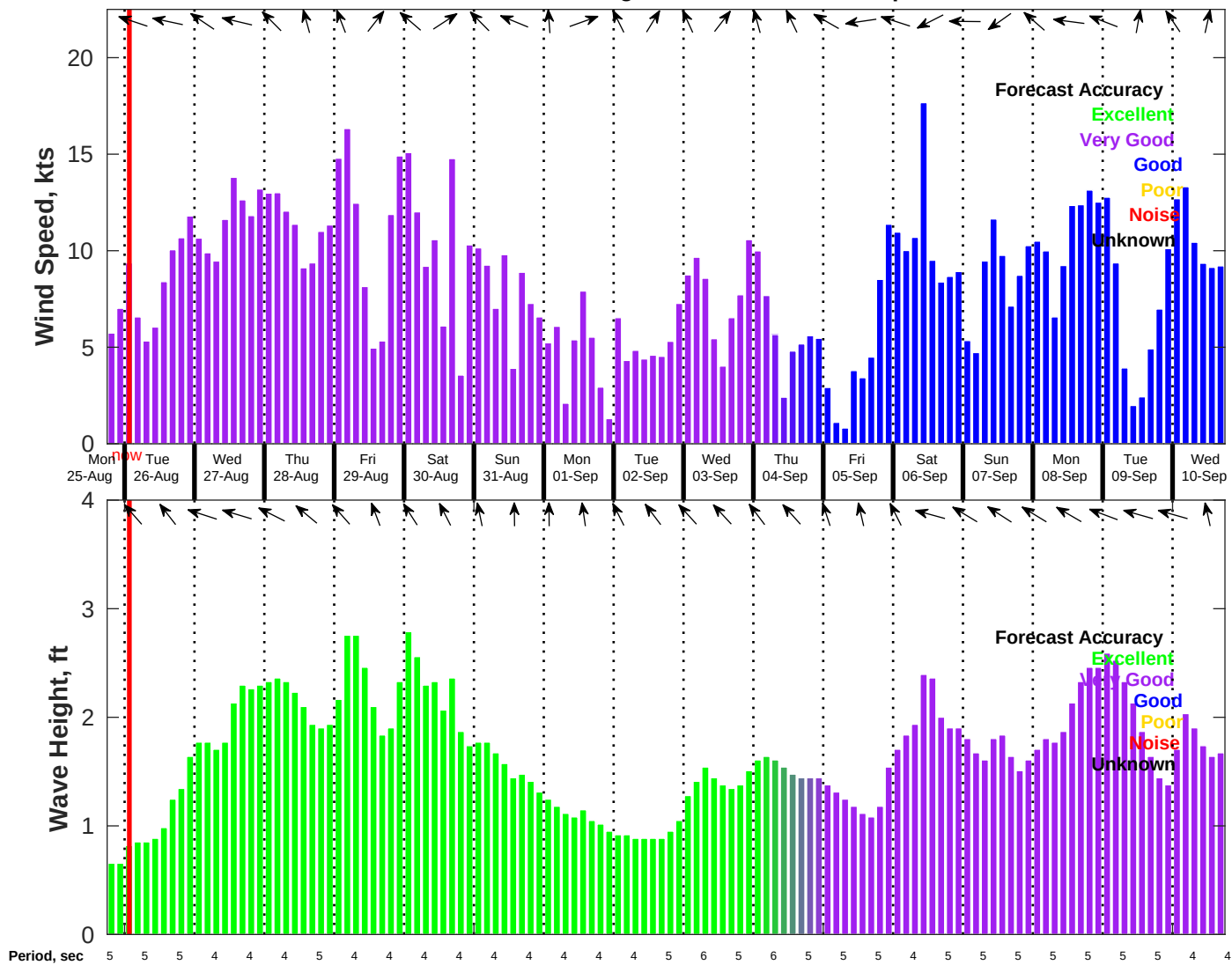
Wind & Wave Forecast for NDBC 42035 from 25-Aug-2025 18:00:00 to 10-Sep-2025 18:00:00
