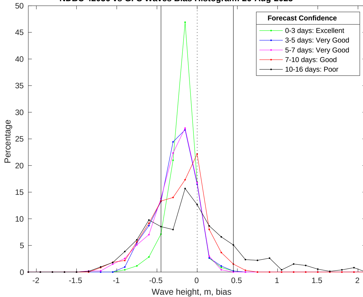
NDBC 42036 vs GFS Waves Bias Histogram: 26-Aug-2025
