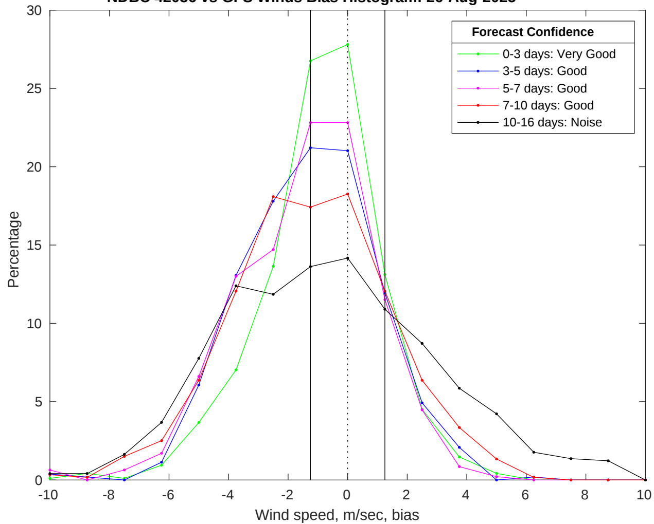
NDBC 42036 vs GFS Winds Bias Histogram: 26-Aug-2025
