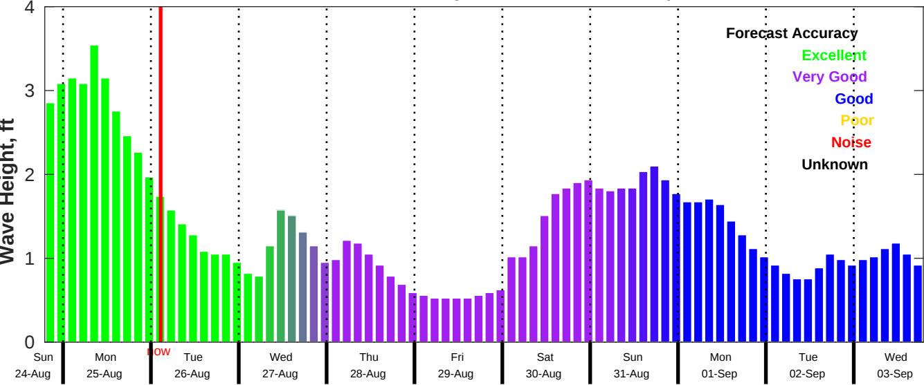
CMEMS Wave Forecast for NDBC 42036 from 24-Aug-2025 19:00:00 to 03-Sep-2025 19:00:00
