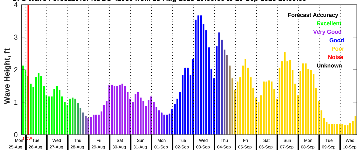
GFS Wave Forecast for NDBC 42036 from 25-Aug-2025 19:00:00 to 10-Sep-2025 19:00:00
