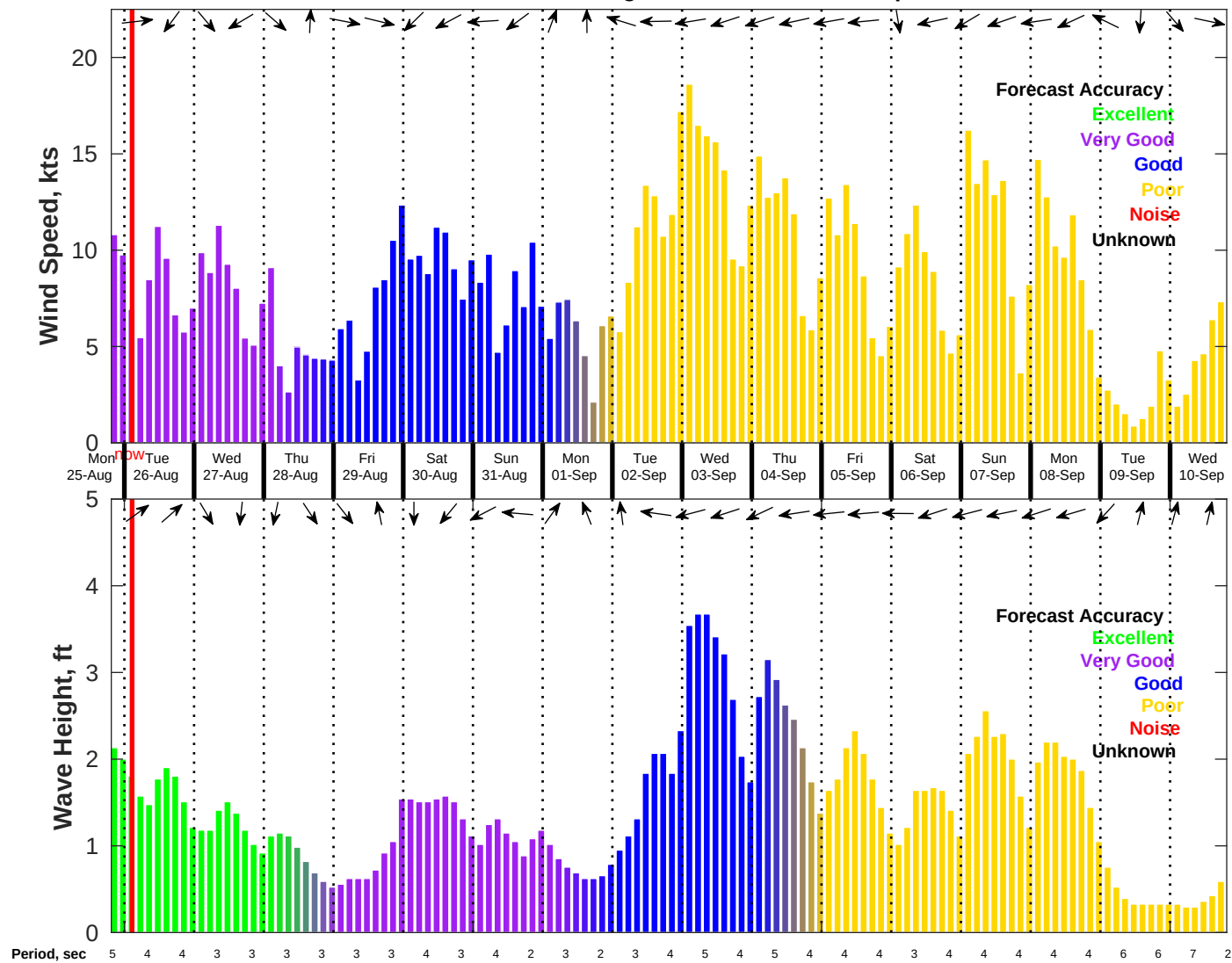
Wind & Wave Forecast for NDBC 42036 from 25-Aug-2025 19:00:00 to 10-Sep-2025 19:00:00
