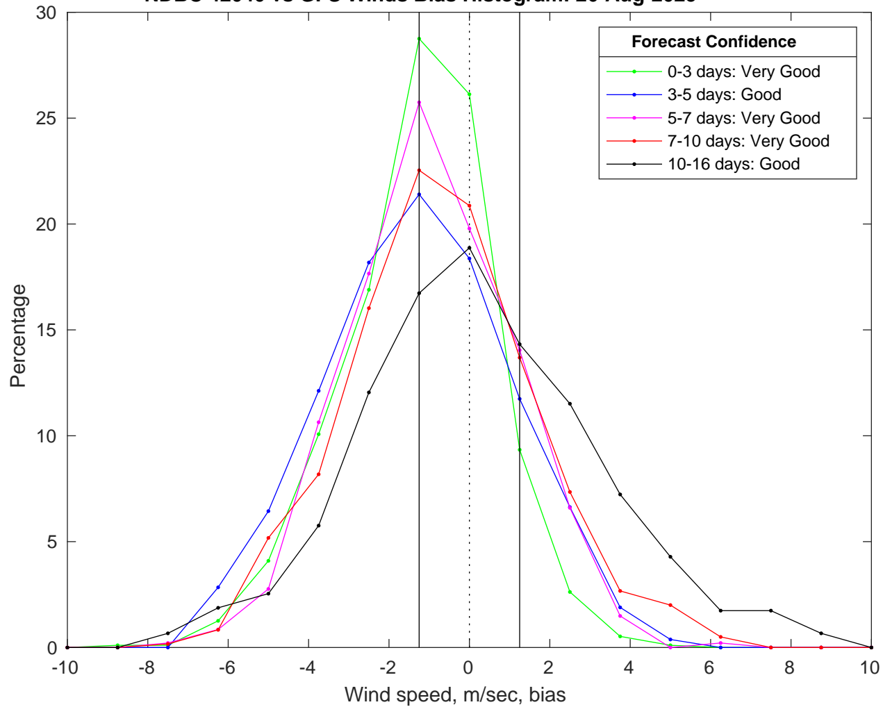
NDBC 42040 vs GFS Winds Bias Histogram: 26-Aug-2025
