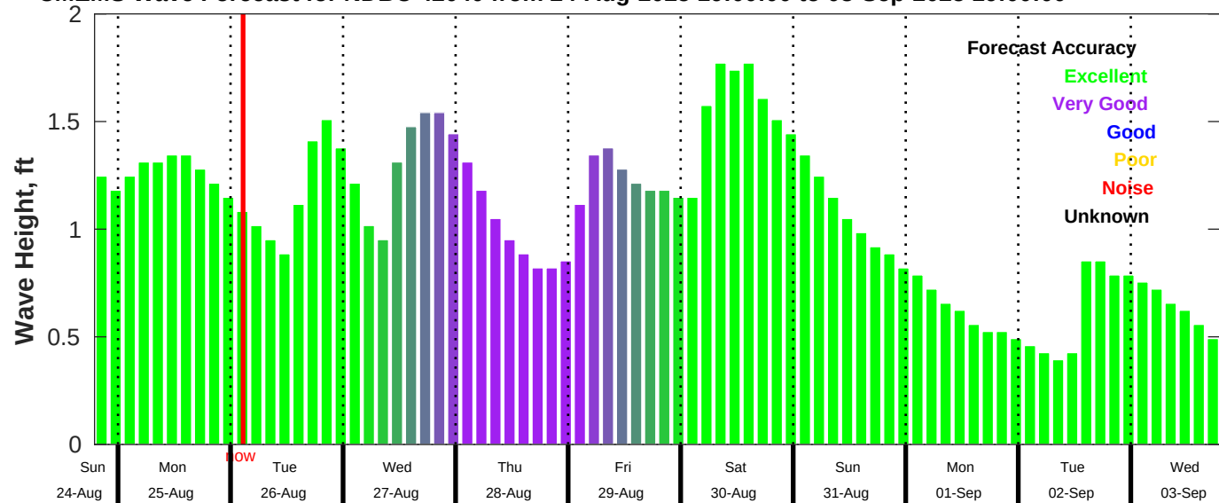
CMEMS Wave Forecast for NDBC 42040 from 24-Aug-2025 19:00:00 to 03-Sep-2025 19:00:00
