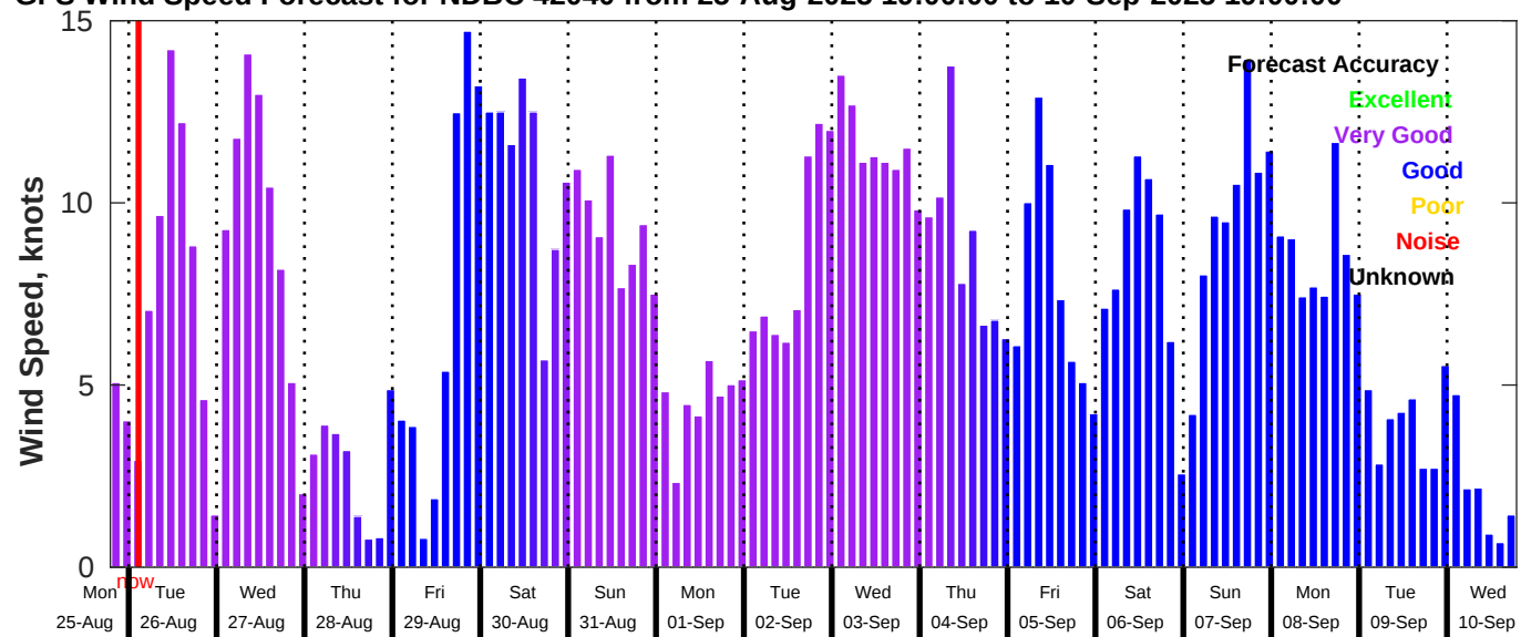
GFS Wind Speed Forecast for NDBC 42040 from 25-Aug-2025 19:00:00 to 10-Sep-2025 19:00:00
