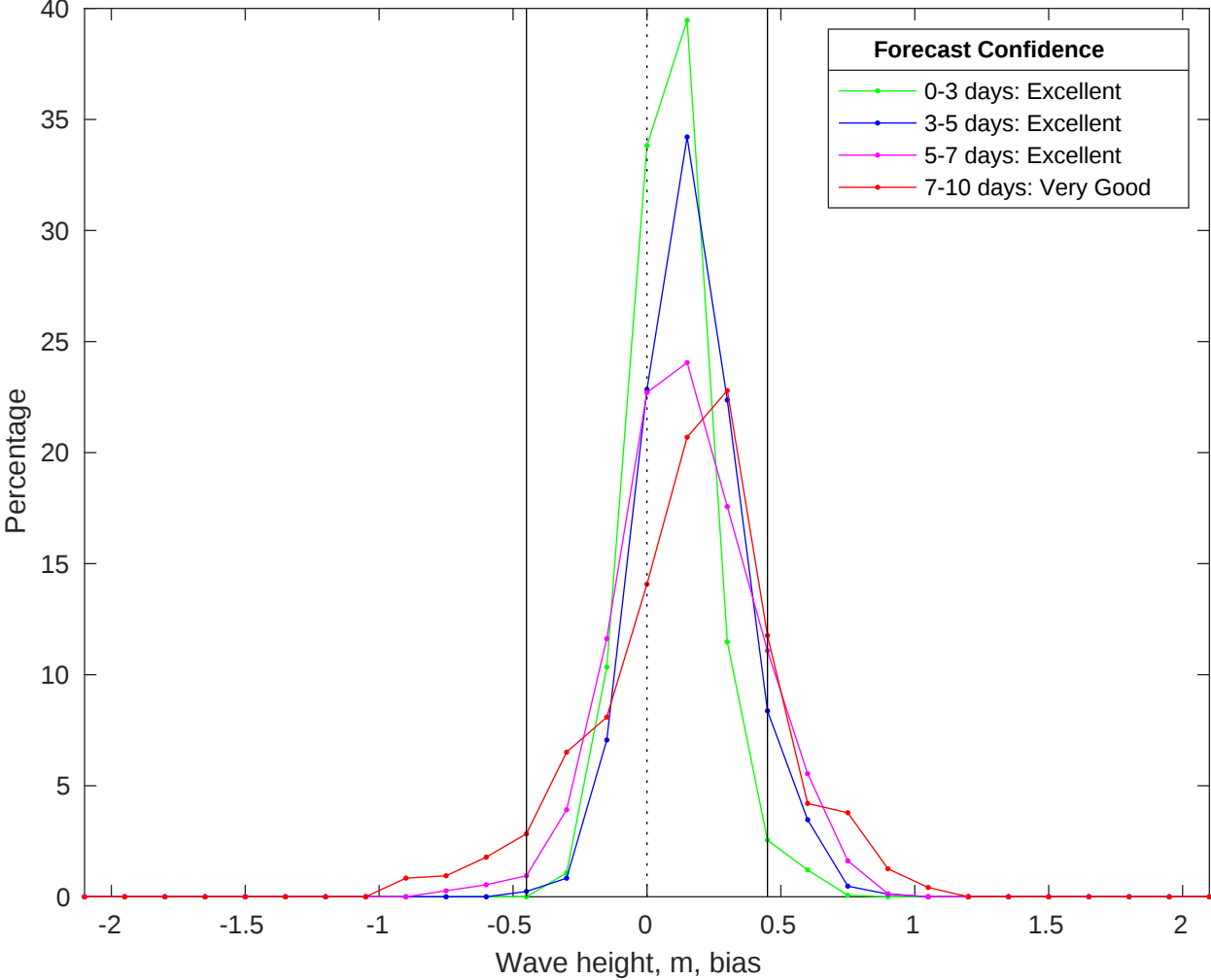
NDBC 46011 vs CMEMS Waves Bias Histogram: 26-Aug-2025
