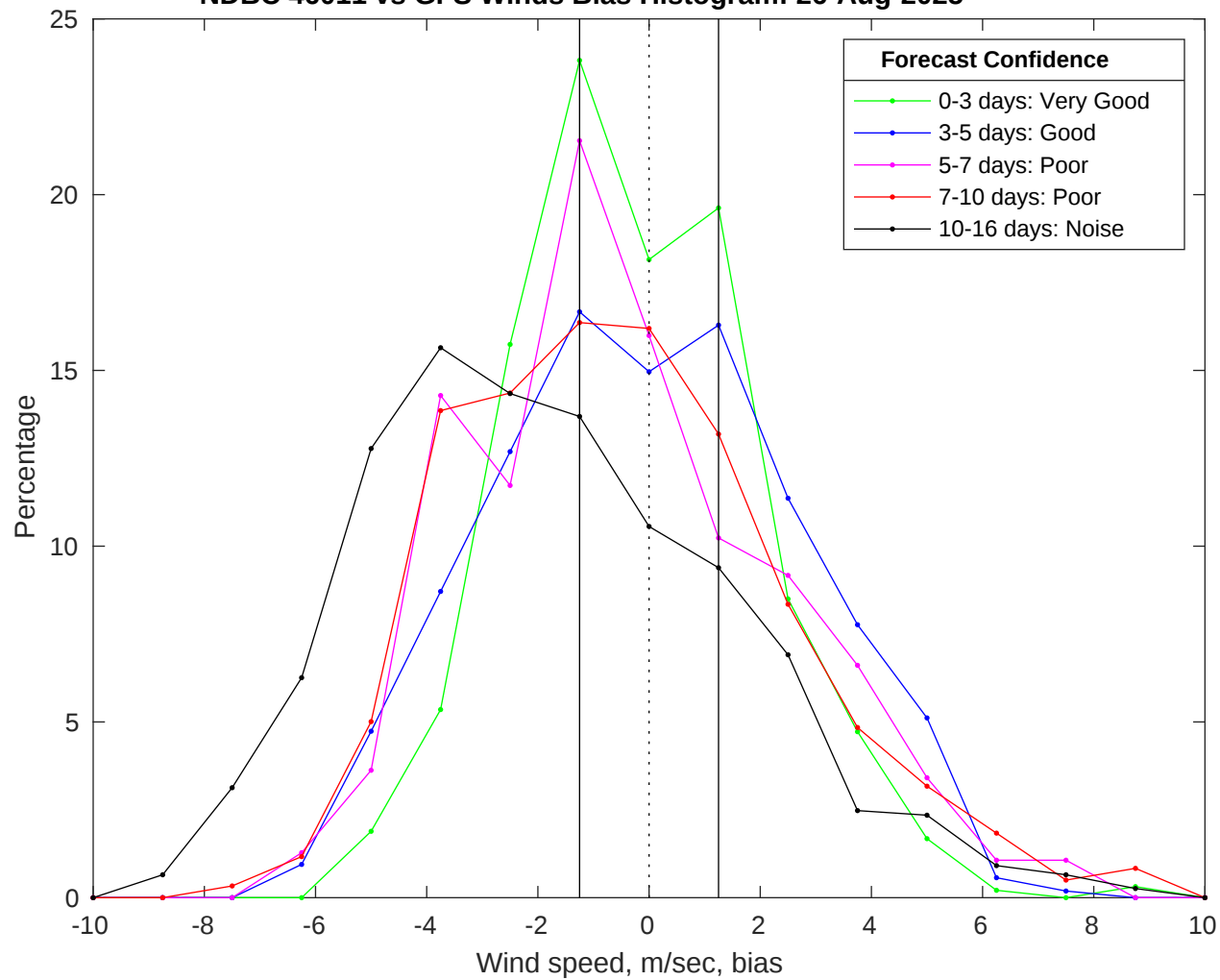
NDBC 46011 vs GFS Winds Bias Histogram: 26-Aug-2025
