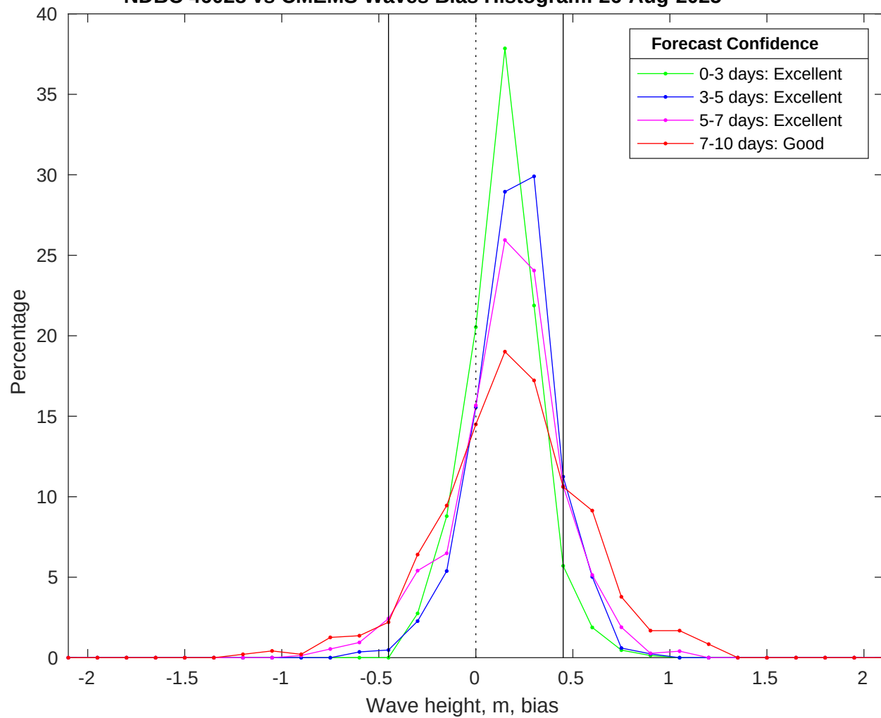
NDBC 46028 vs CMEMS Waves Bias Histogram: 26-Aug-2025
