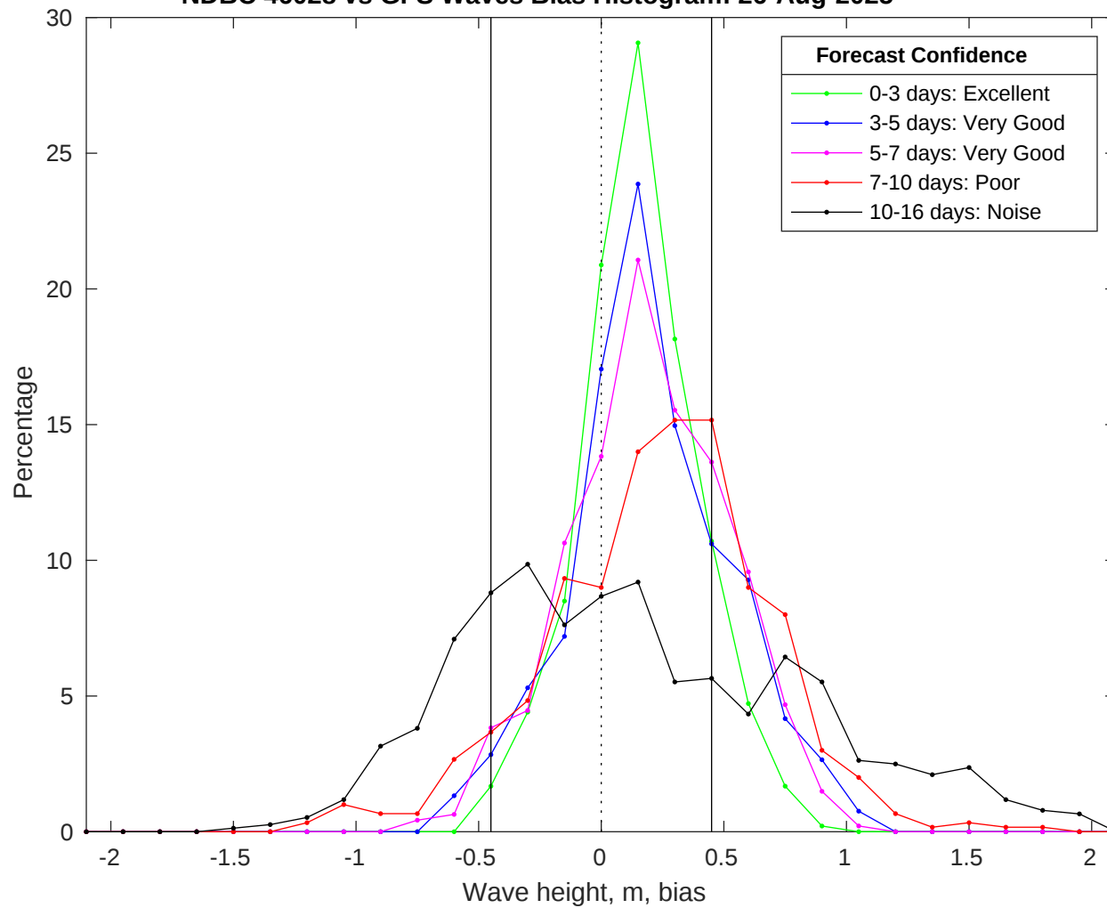
NDBC 46028 vs GFS Waves Bias Histogram: 26-Aug-2025
